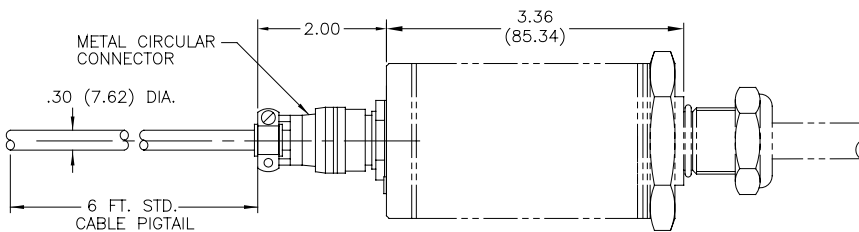
CONNECTOR OPTION E 10 PIN CIRCULAR
